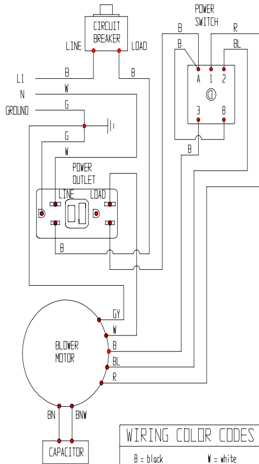
SAHARA PRO X3 - 115V 60HZ WIRING DIAGRAM
